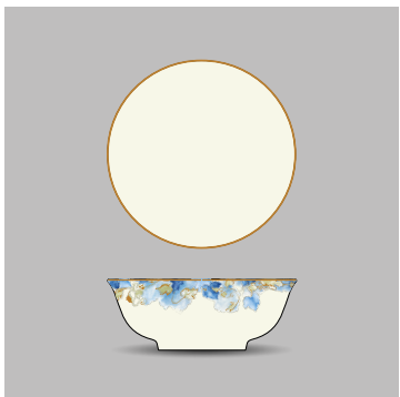
5013519 NOODLE SOUP BOWL 19 CM. Ø 195 mm. Height 74.5 mm. Capacity 1,110 cc. (39 oz.)
